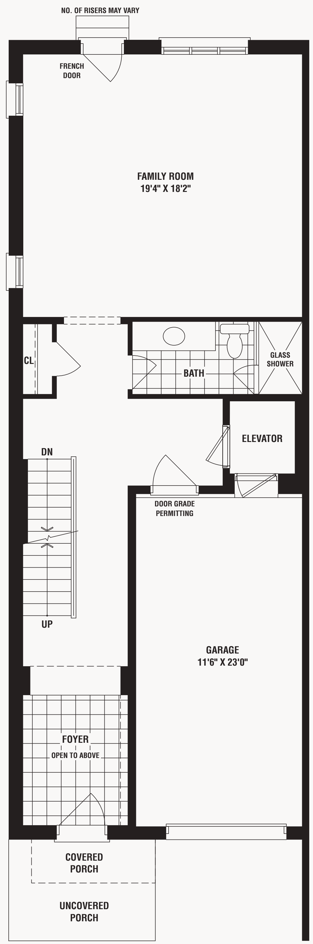
GROUND FLOOR PLAN ELEV. 'A' END
