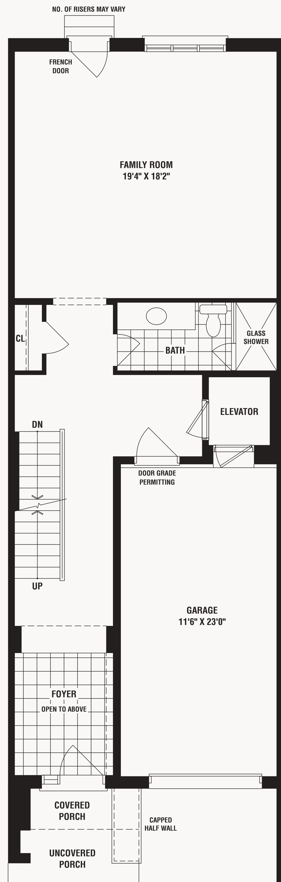
GROUND FLOOR PLAN ELEV. 'A'
