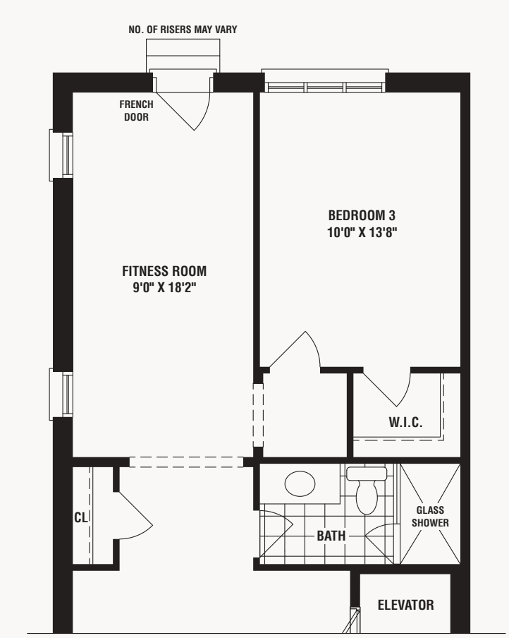
PARTIAL ALT. GROUND FLOOR PLAN W/ BEDROOM 3
