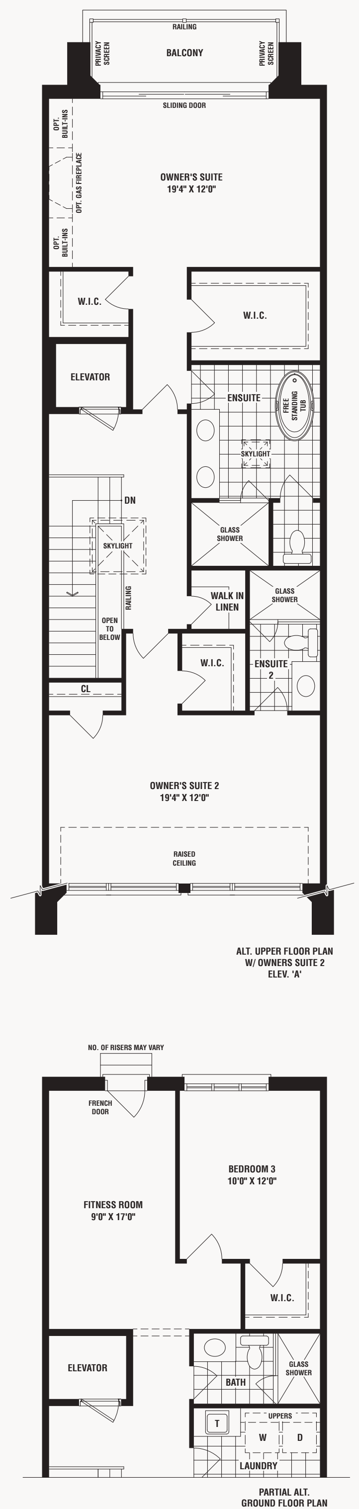
PARTIAL ALT. GROUND FLOOR PLAN
