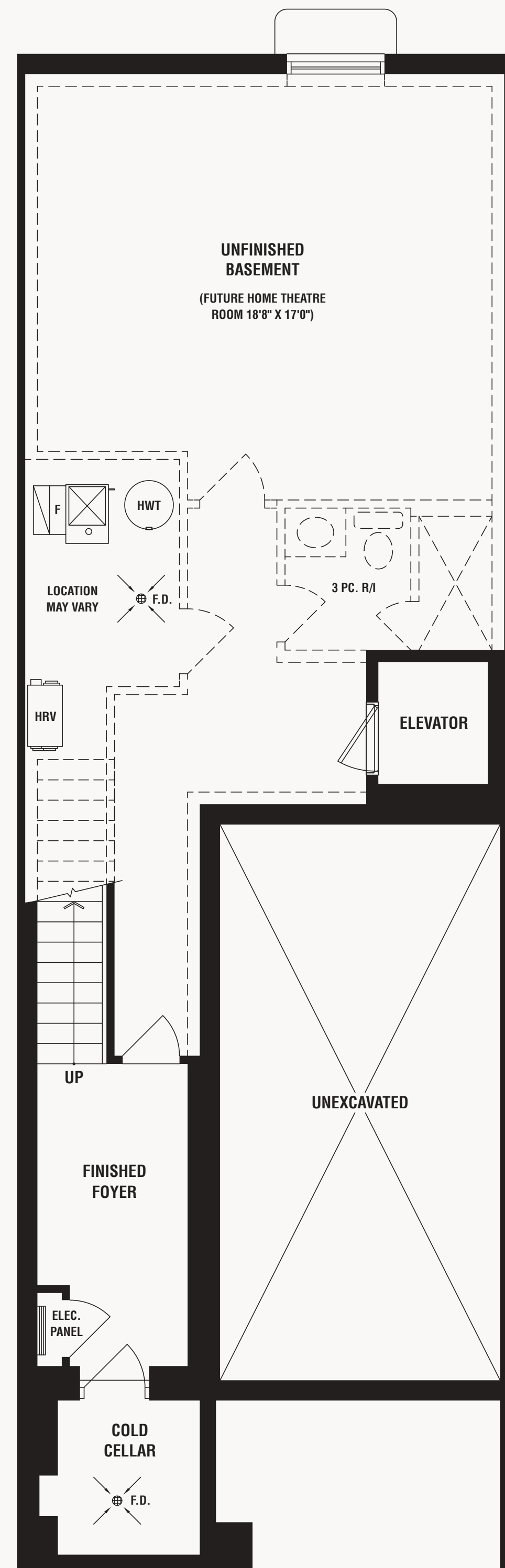
BASEMENT PLAN ELEV. 'A'
