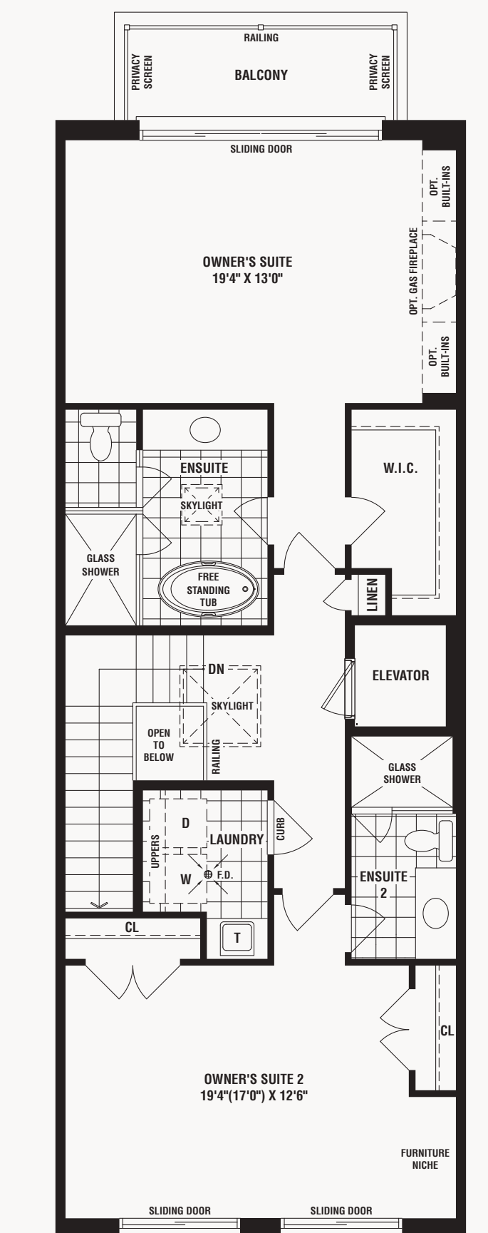
ALT. UPPER FLOOR PLAN W/ OWNER'S SUITE 2 ELEV. 'A'
