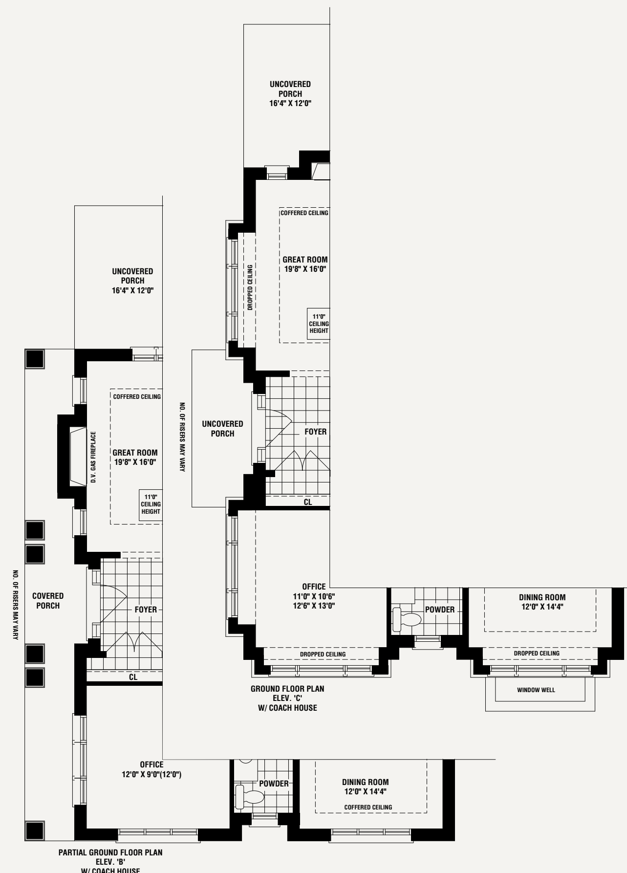
PARTIAL GROUND FLOOR PLAN ELEV. 'B' W/ COACH HOUSE
