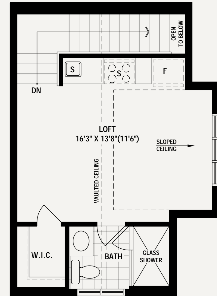
COACH HOUSE ELEV. 'A7/B7/C'
