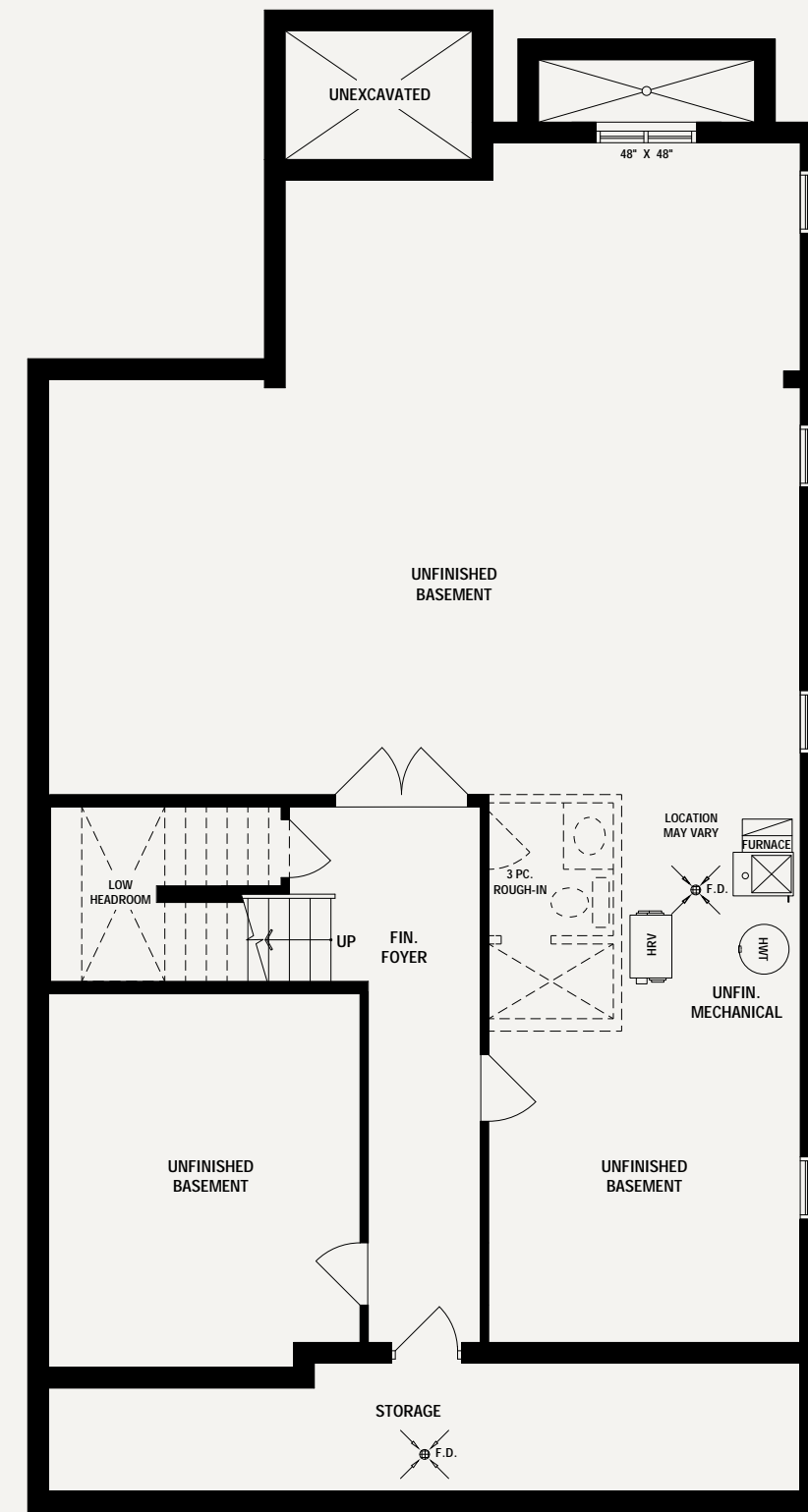
BASEMENT ELEV. 'A7/B'
