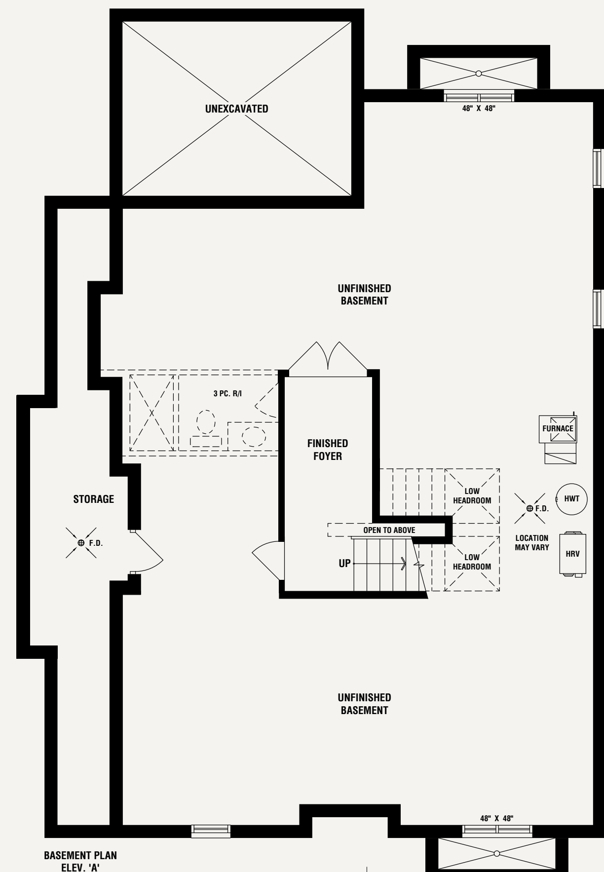
BASEMENT PLAN ELEV. 'A'
