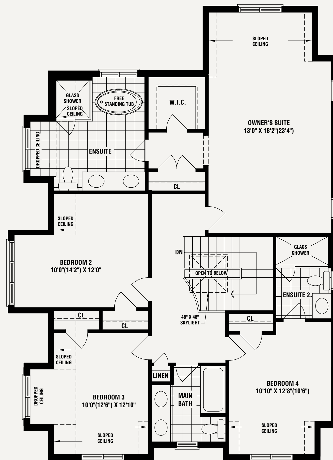
SECOND FLOOR PLAN ELEV. 'A'
