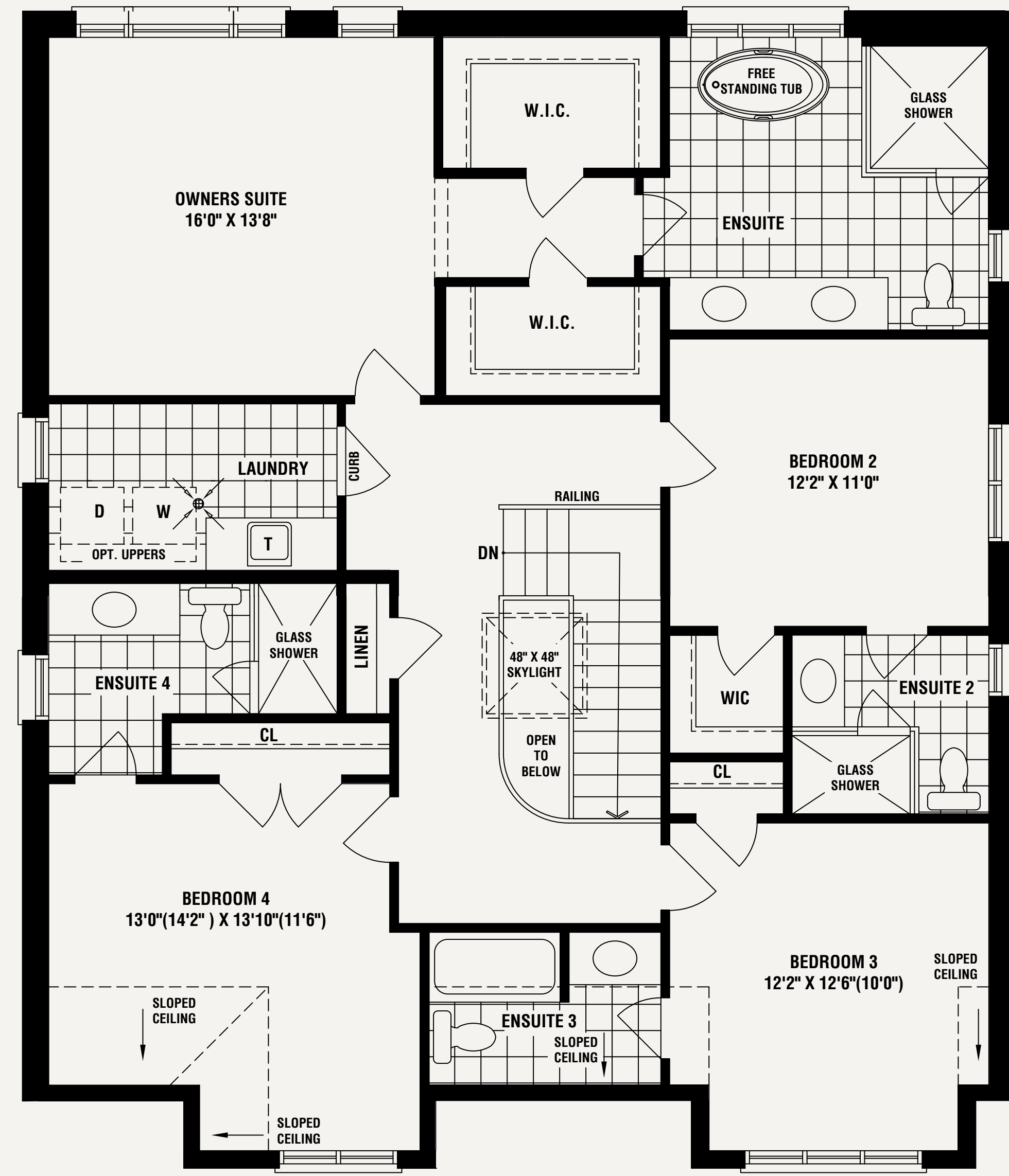
SECOND FLOOR ELEV. 'A'
